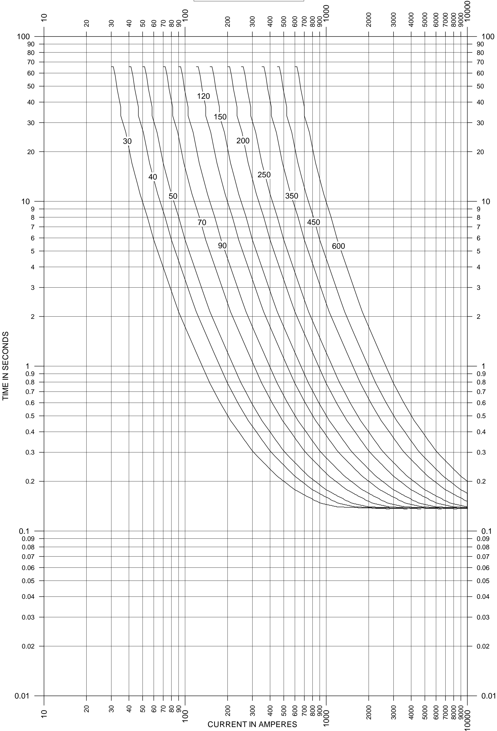
Relay Curve 30 - 600 CO-11-3
