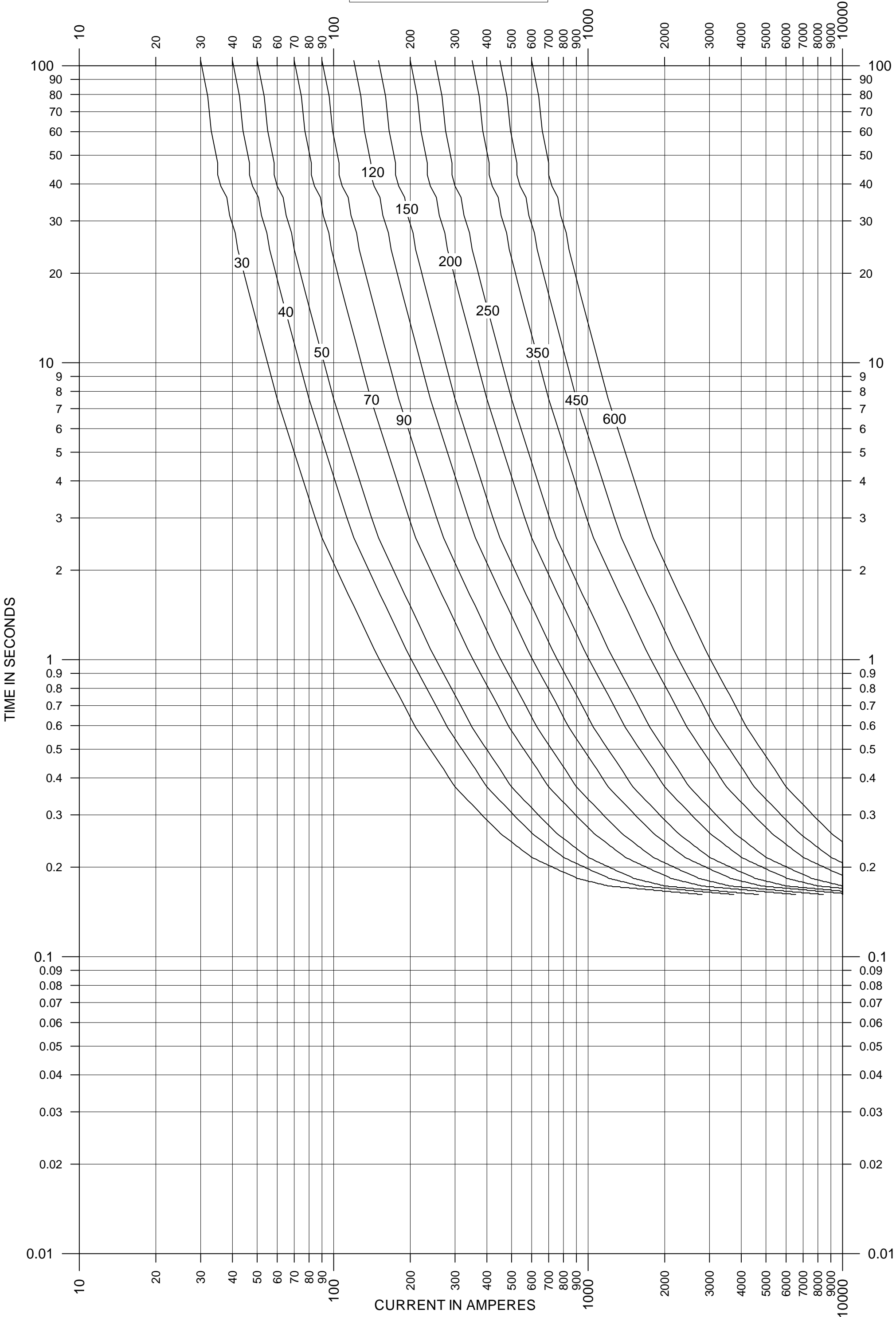
Relay Curve 30 - 600 CO-11-4
