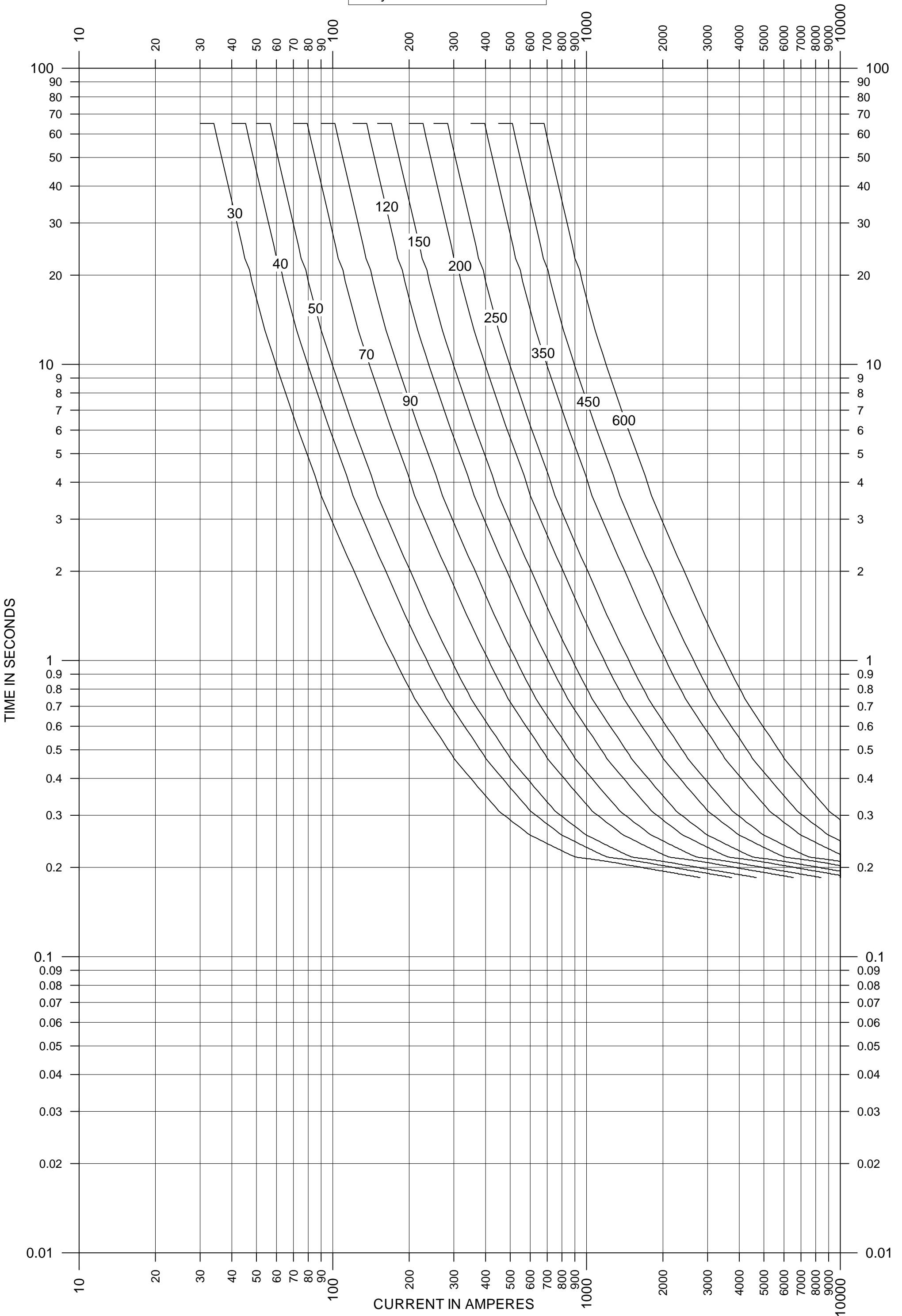
Relay Curve 30 - 600 CO-11-5
