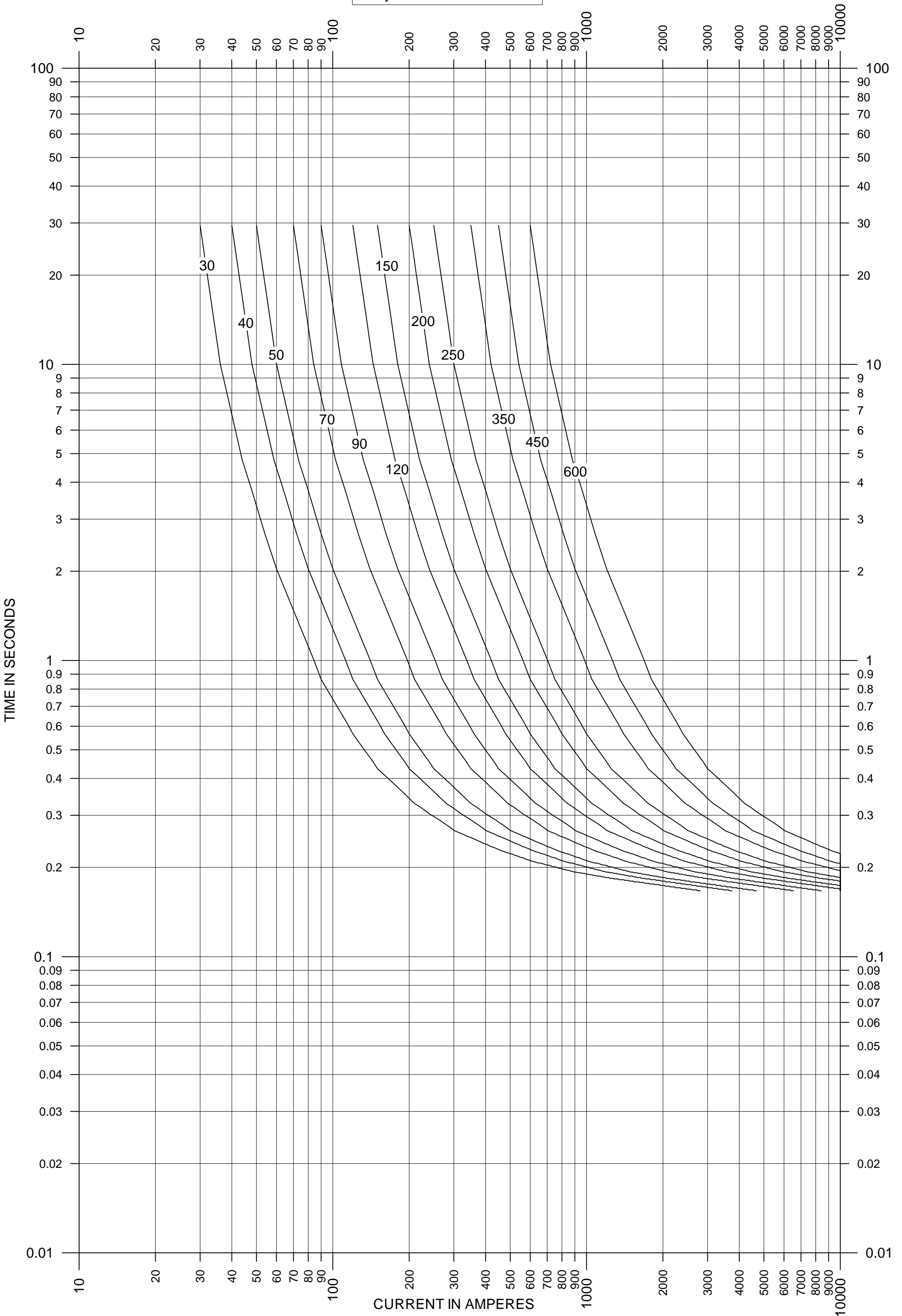
Relay Curve 30 - 600 CO-8-1
