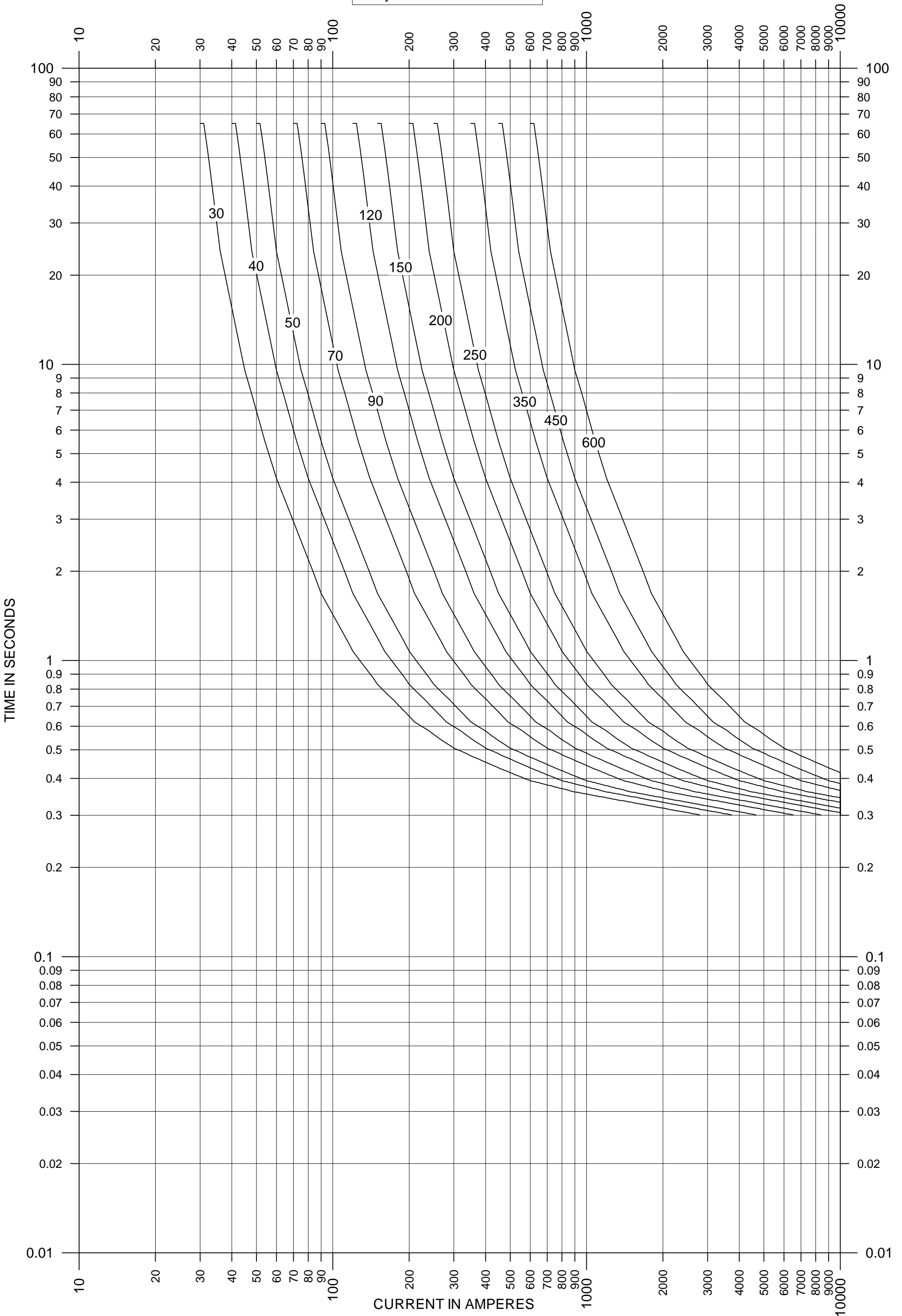
Relay Curve 30 - 600 CO-8-2
