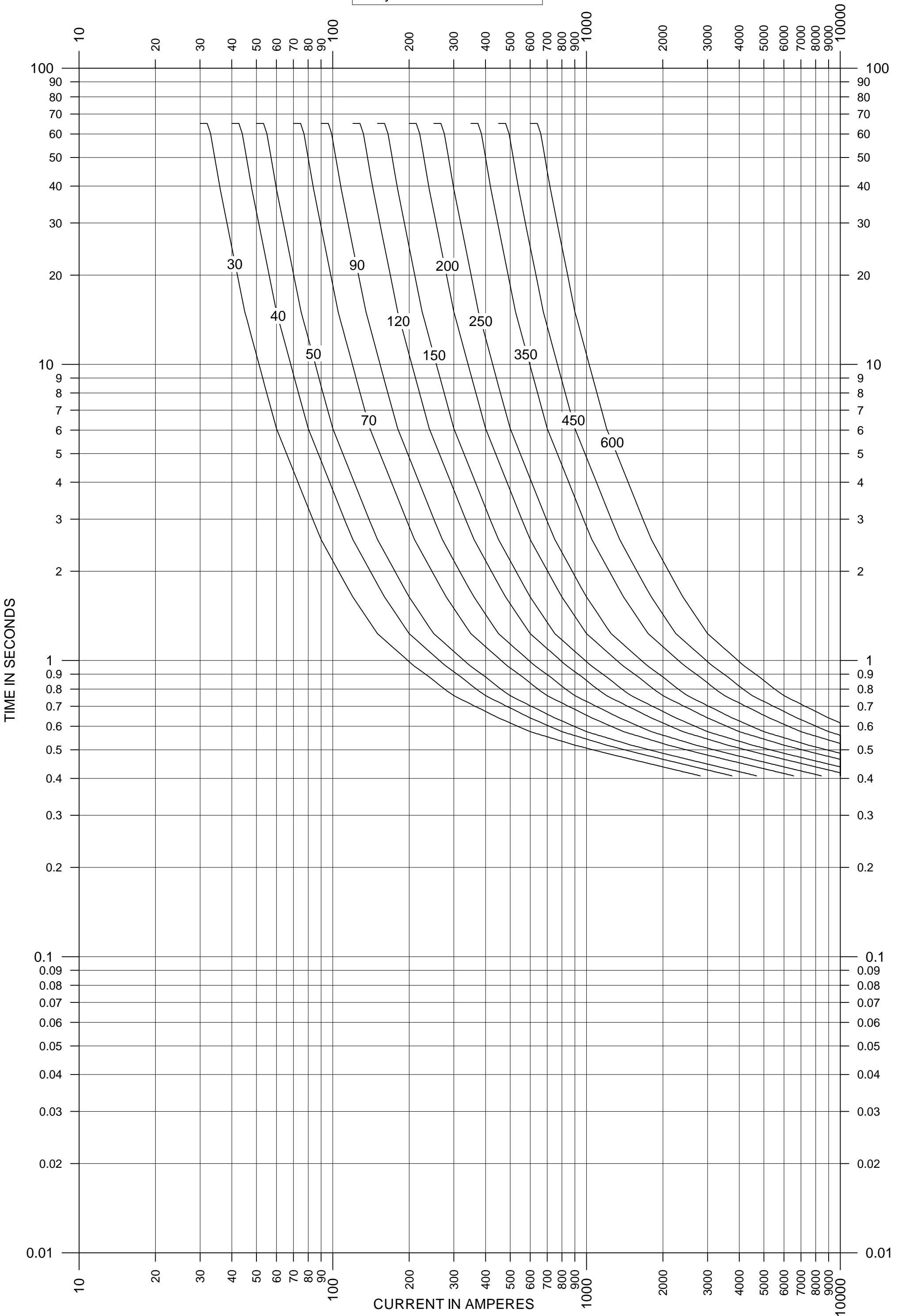
Relay Curve 30 - 600 CO-8-3
