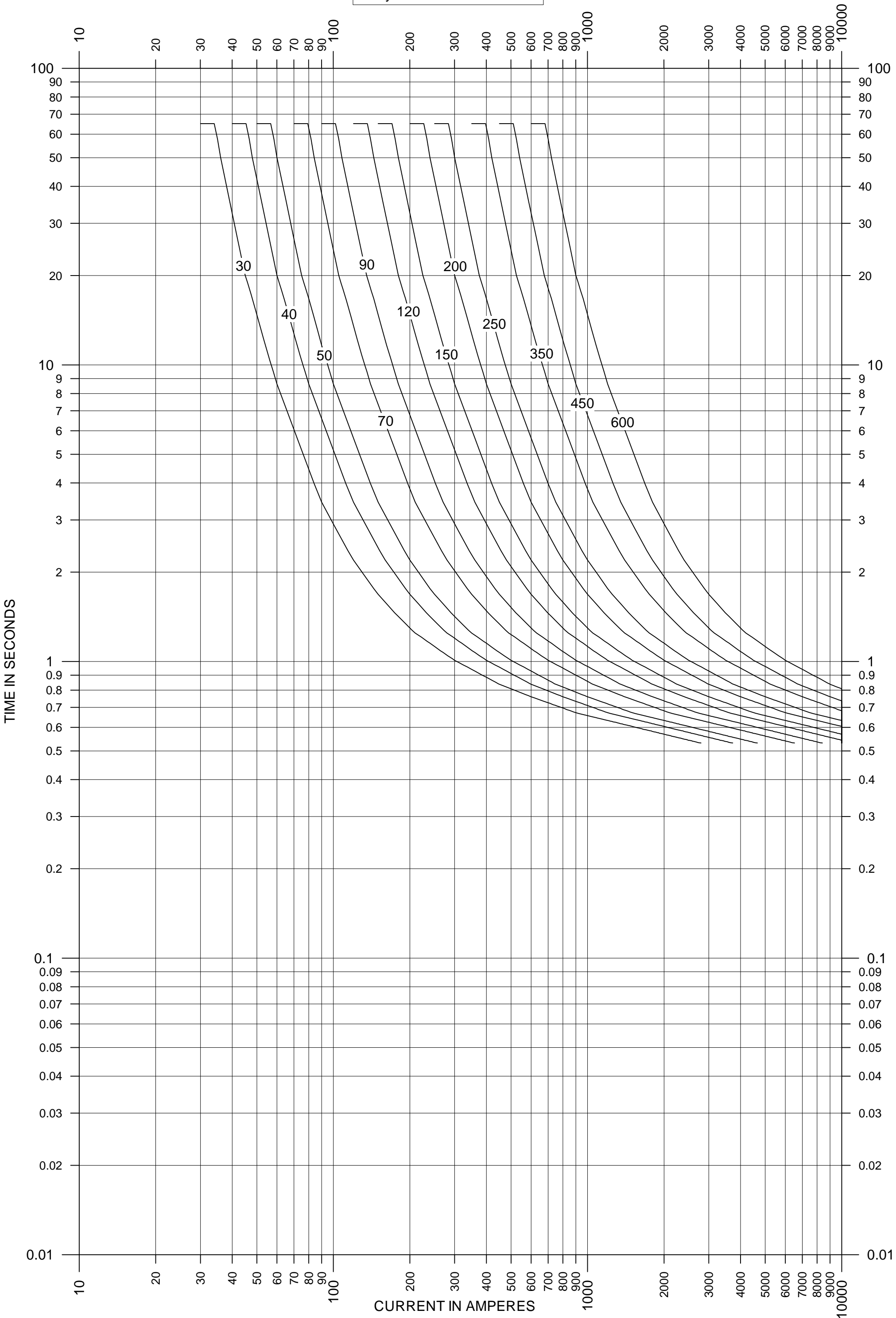
Relay Curve 30 - 600 CO-8-4
