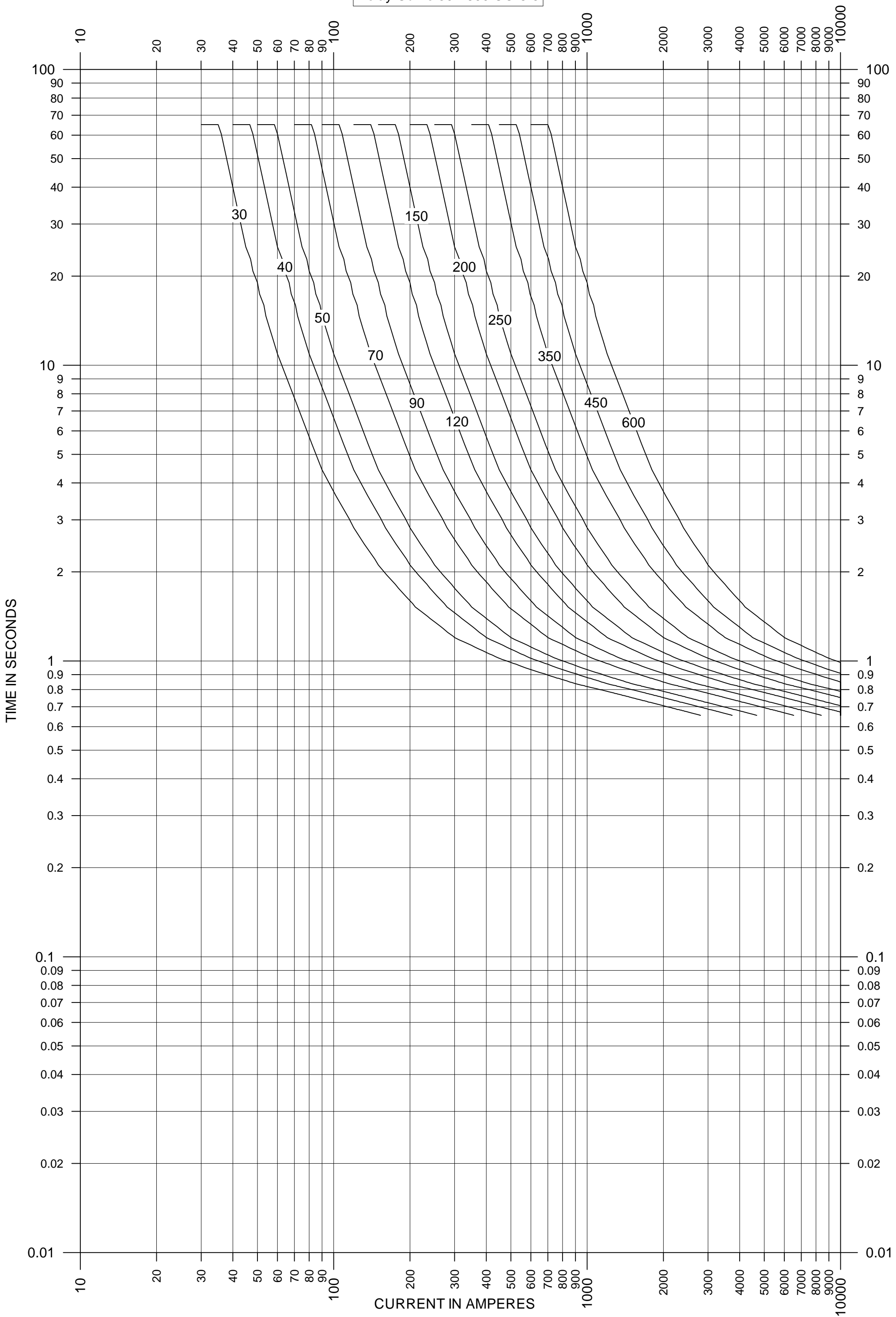
Relay Curve 30 - 600 CO-8-5
