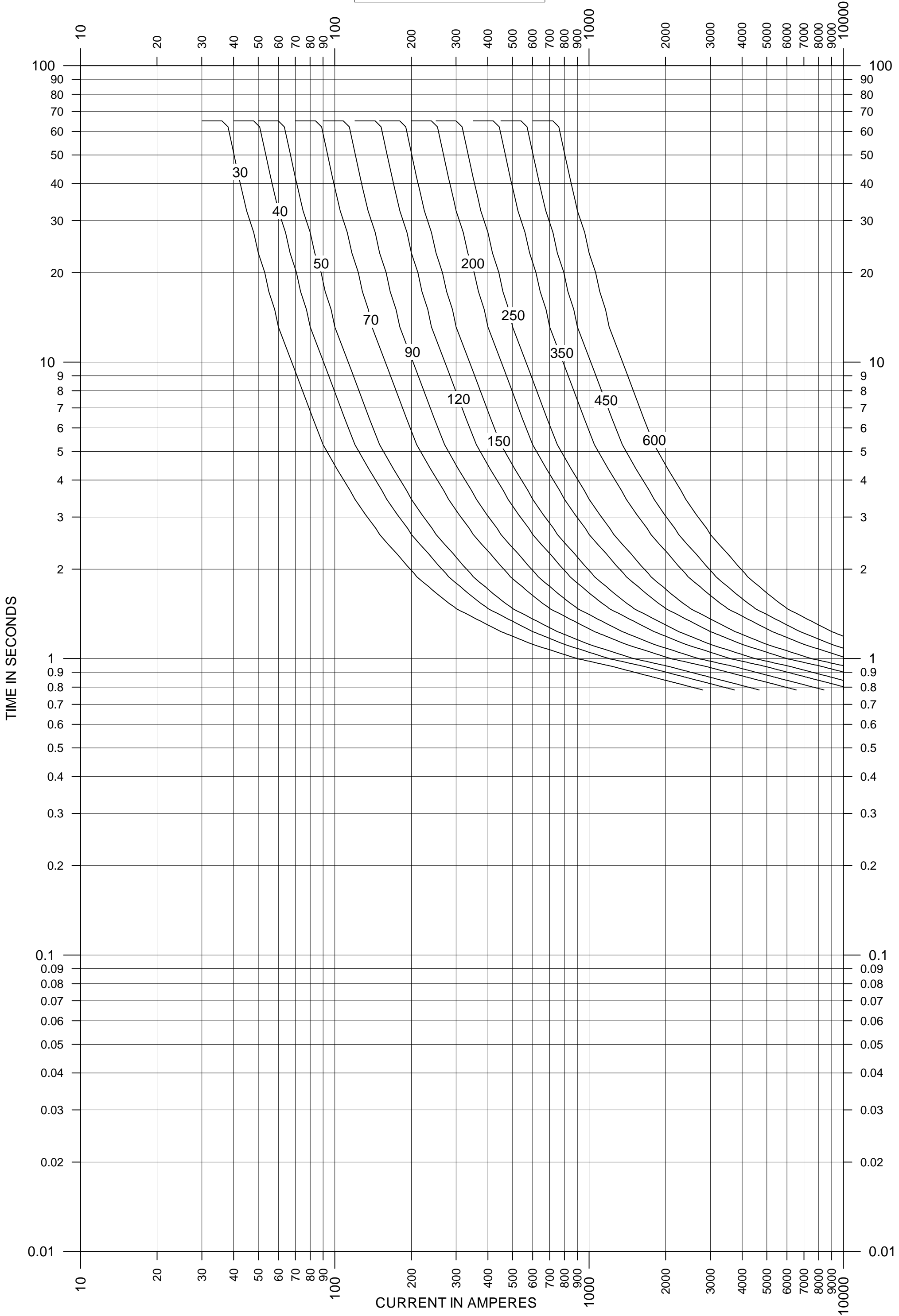
Relay Curve 30 - 600 CO-8-6
