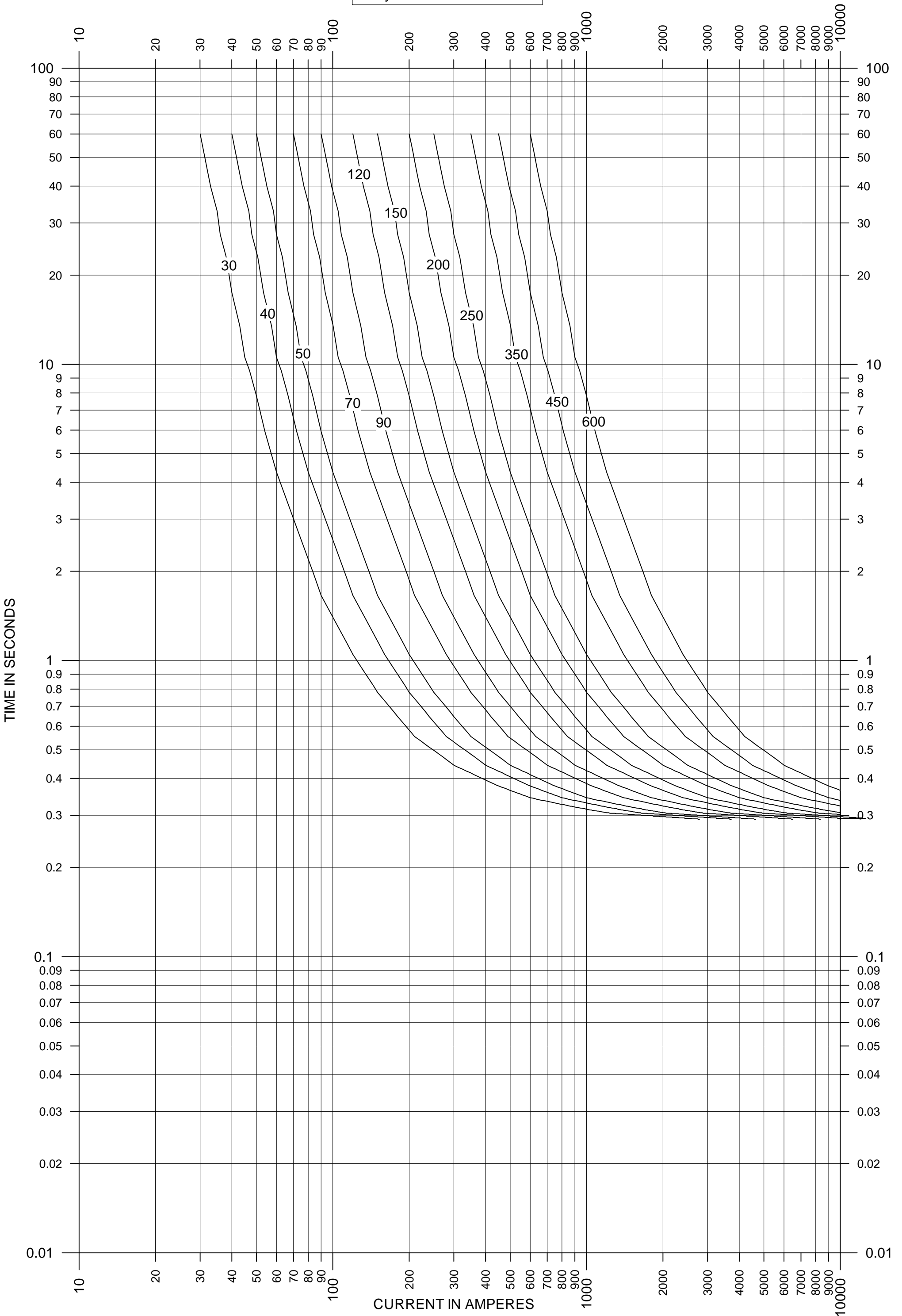
Relay Curve 30 - 600 CO-9-3
