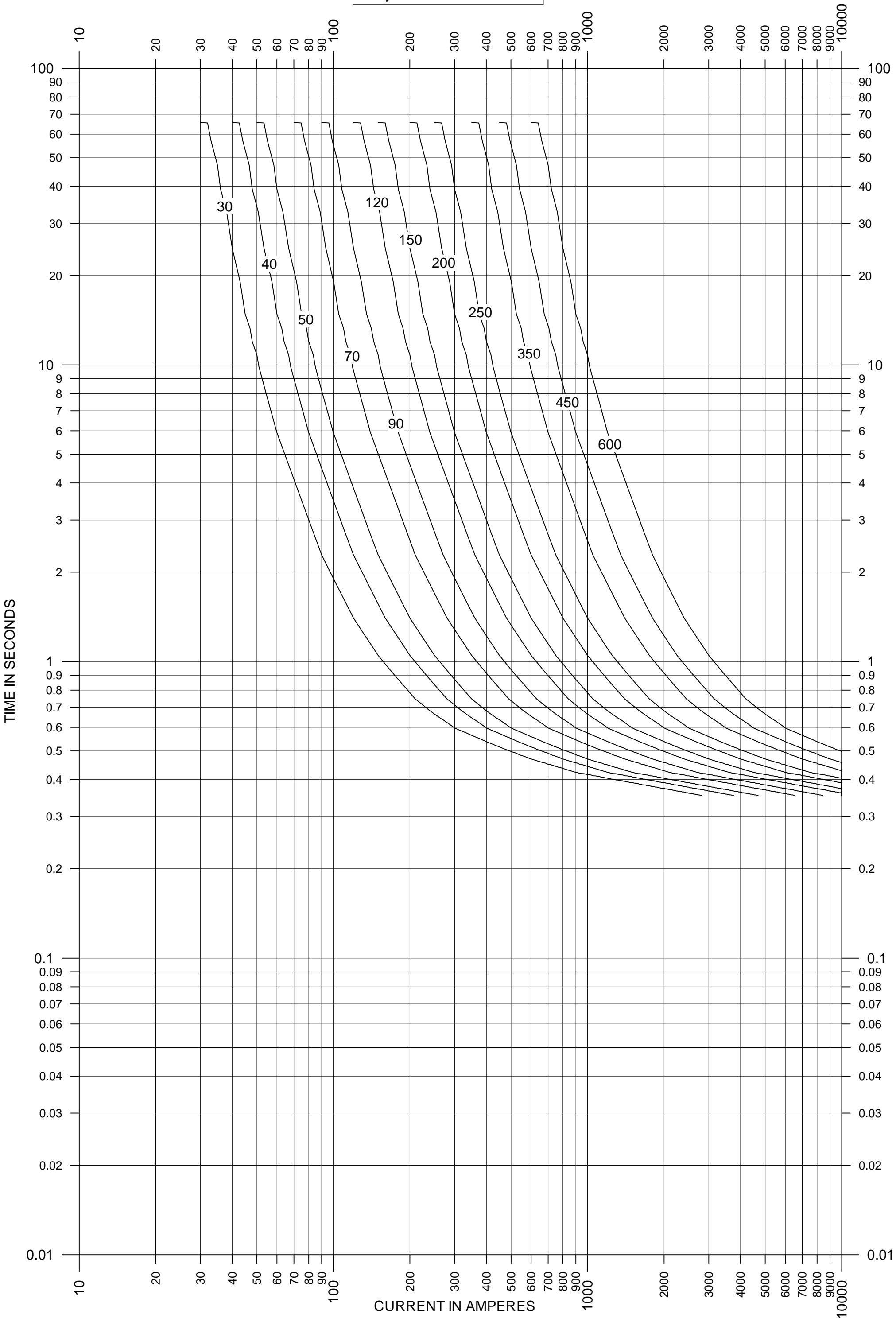
Relay Curve 30 - 600 CO-9-4
