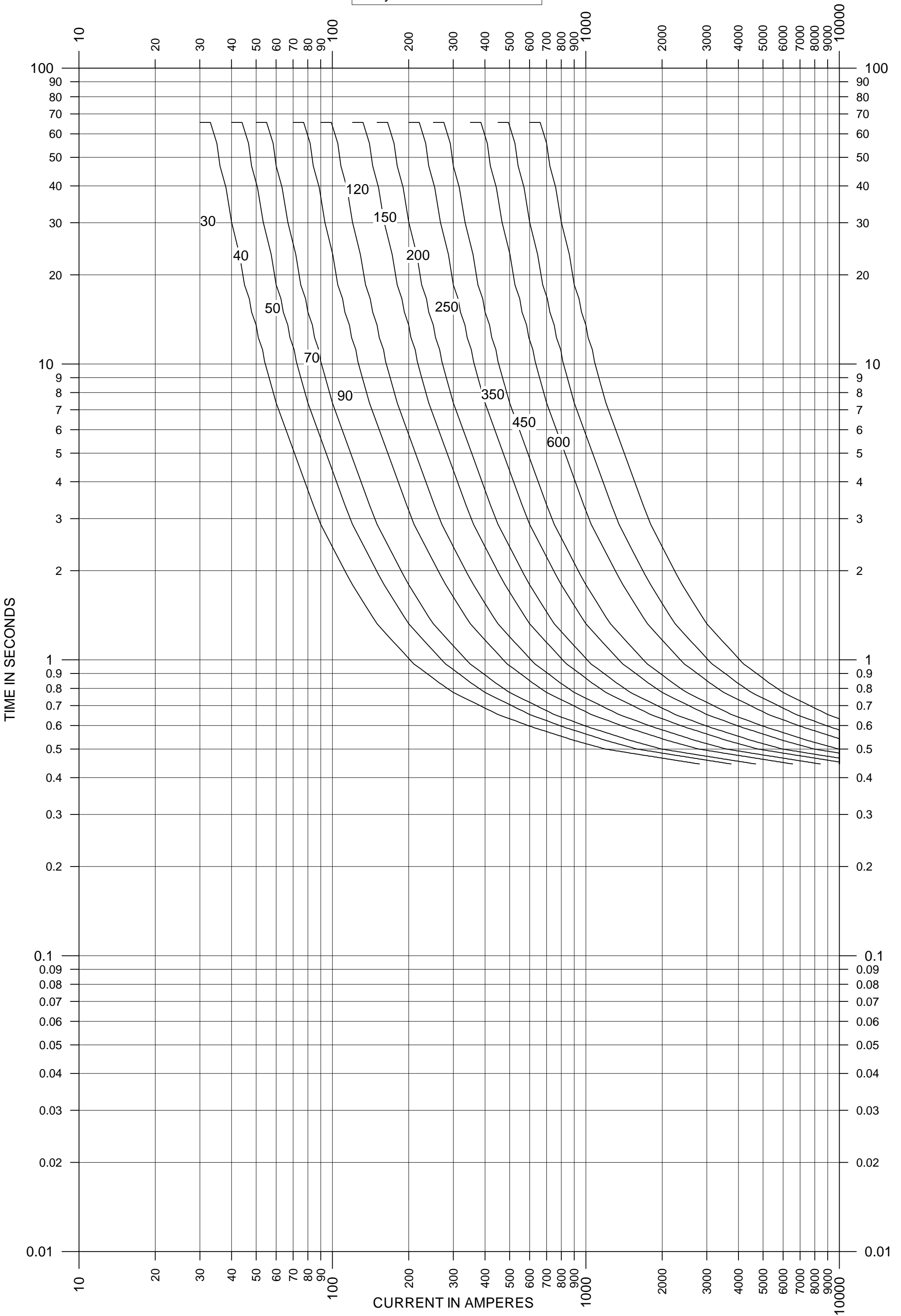
Relay Curve 30 - 600 CO-9-5
