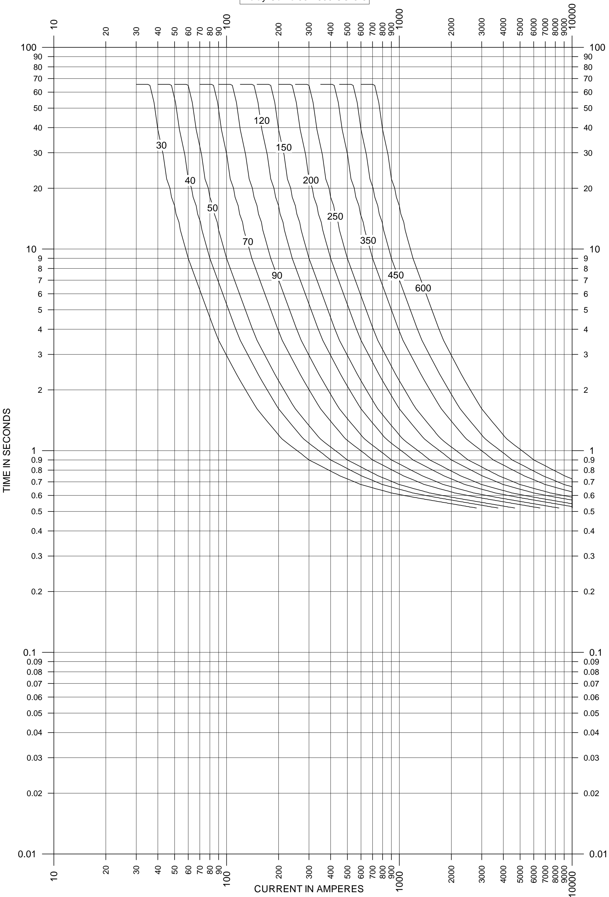
Relay Curve 30 - 600 CO-9-6
