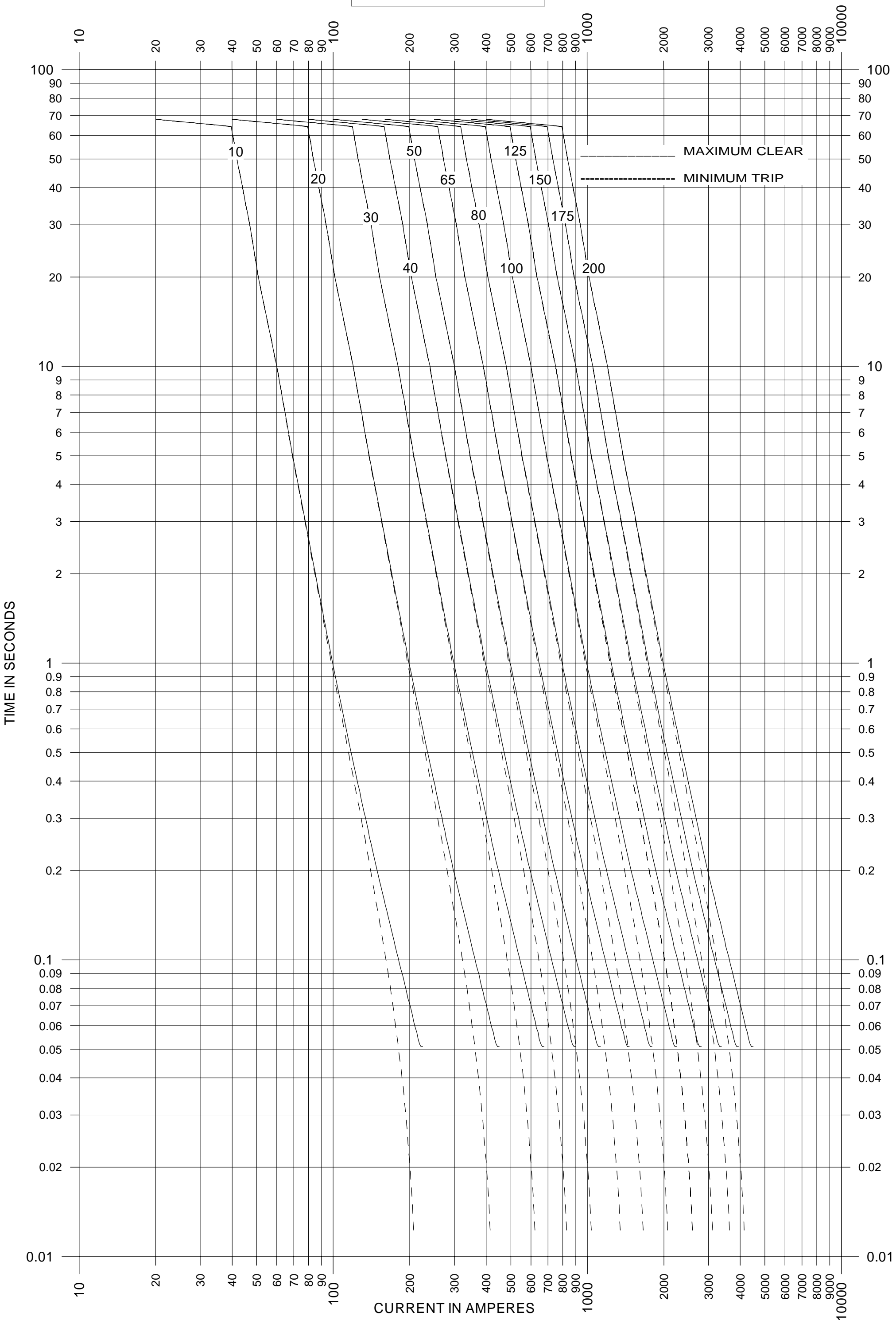
Fuse Curve 10 - 200 NX-35 C
