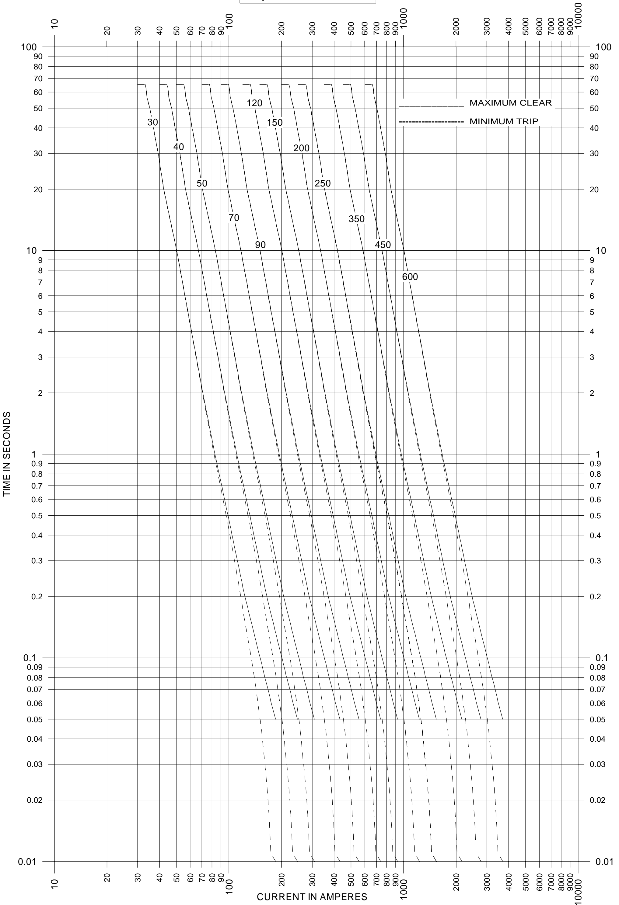
Relay Curve 30 - 600 NX-35 C
